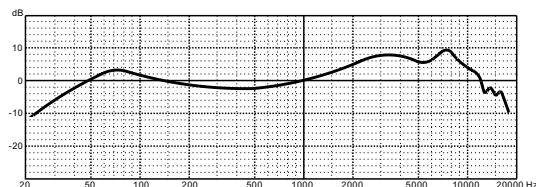
Frequency Response
