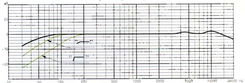
Frequency Response
