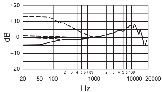
Frequency Response
