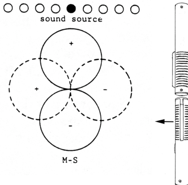
Figure 2 Typical M-S miking technique
