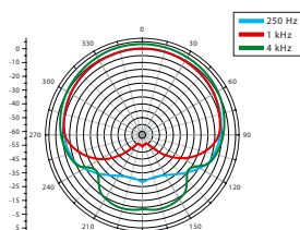
Cardioid
