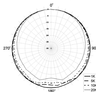
PianoMic™ Polar Response
