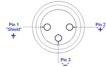
Fig. 1. XLR Output Connector Assignment of QTC30
