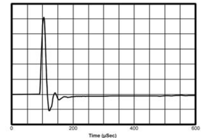
Fig. 3. Impulse Response (Typical) of QTC30
