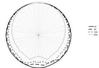
Fig. 4. Polar Response (Typical) of QTC30, 1dB/div.
