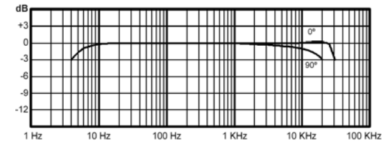
Fig. 2. Frequency Response (Typical) of QTC30
