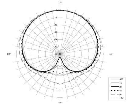
Fig. 4. Polar Response (Typical) of P30/C
