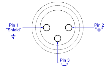
Fig. 1. XLR Output Connector Assignment of P30/C
