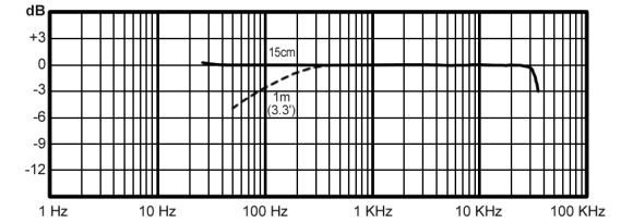
Fig. 2. Frequency Response (Typical) of P30/C
